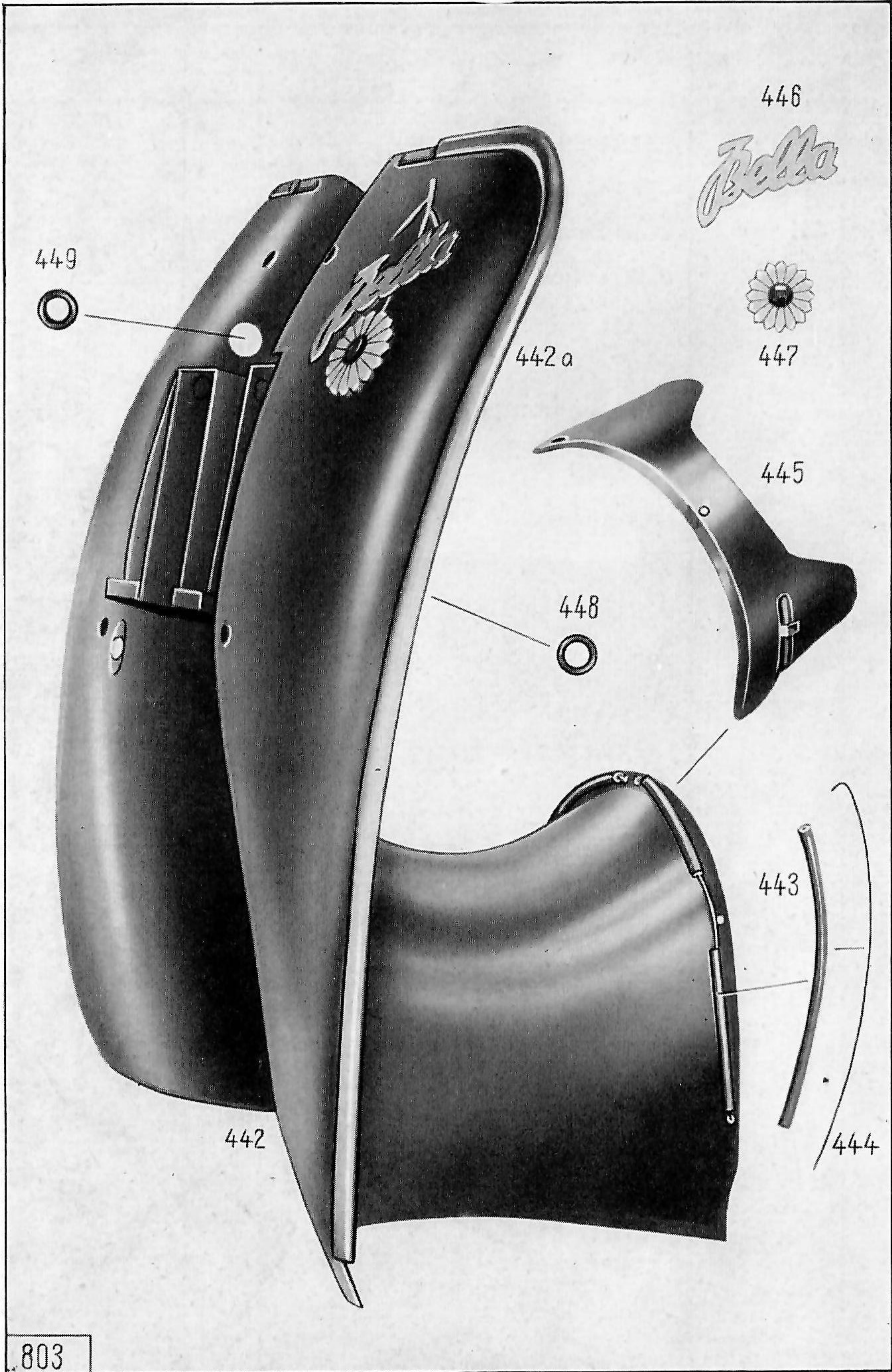
Illustration 17, Group R: e) Front Shield
