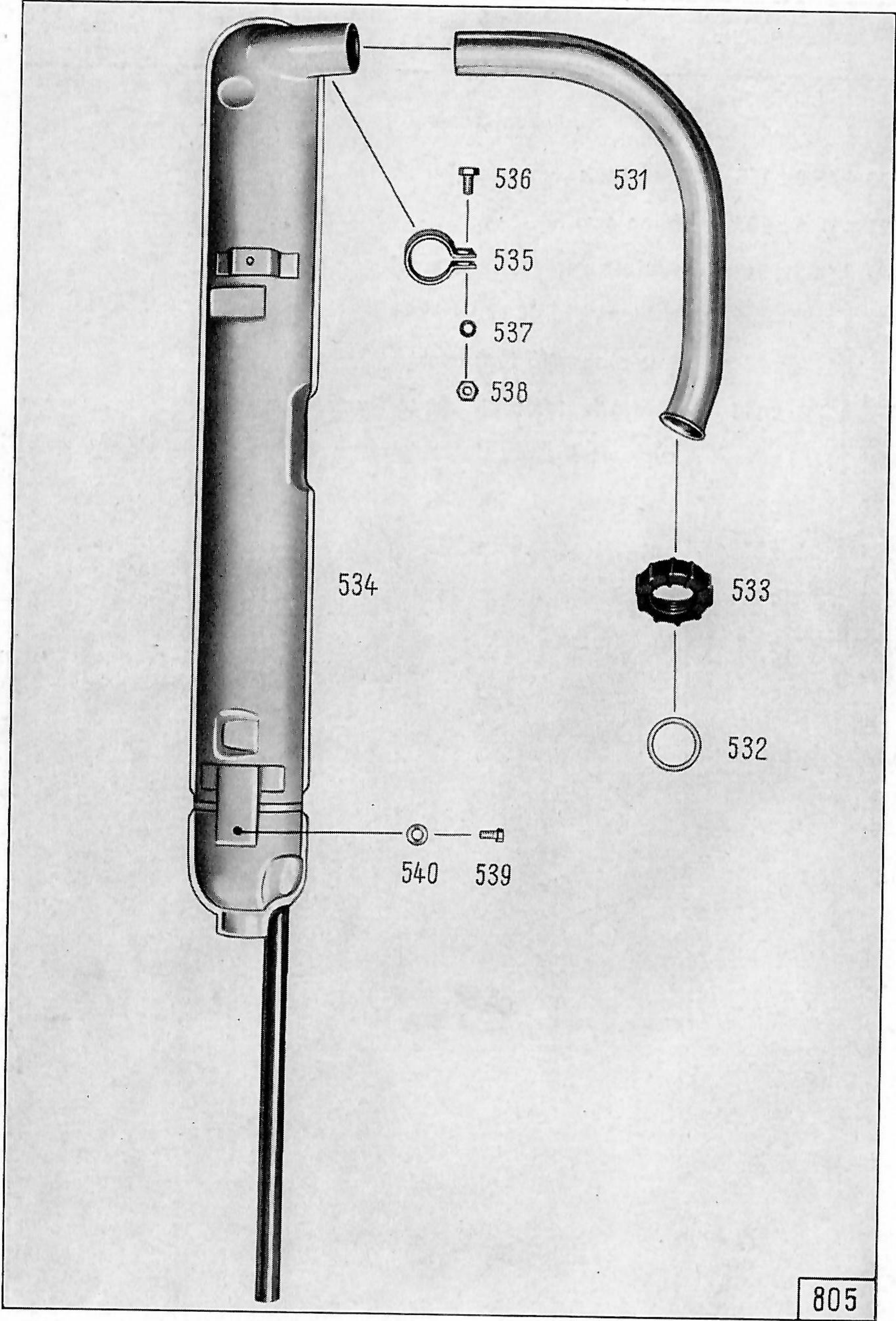
Illustration 22, Group R: h) Exhaust Set
